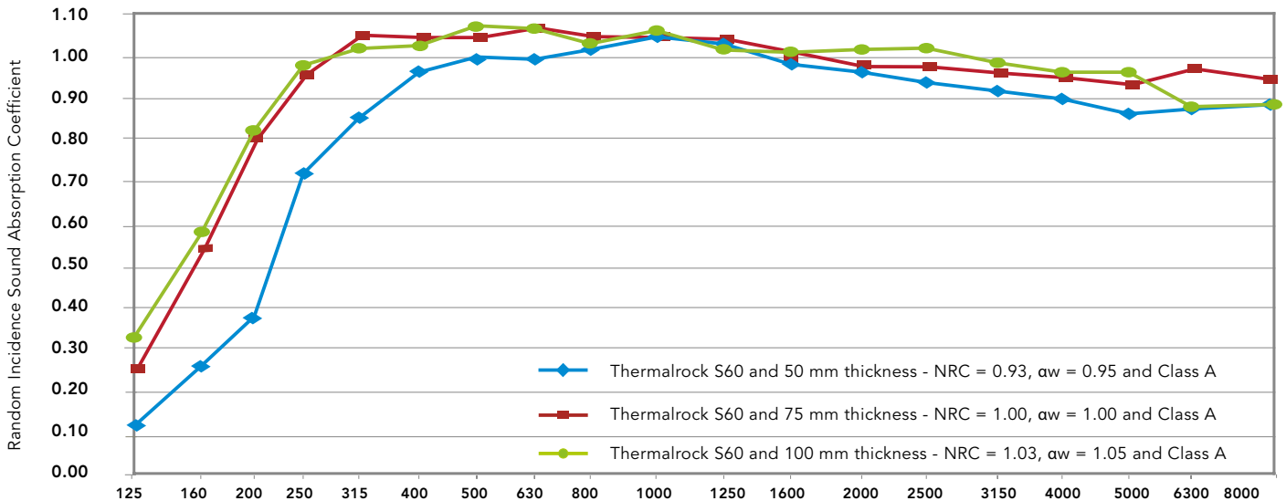
Figure 2: Plot for Random incidence sound absorption coefficient (RISAC) of Thermalrock S60 50 mm, 75 mm and 100 mm at one third octave frequencies
